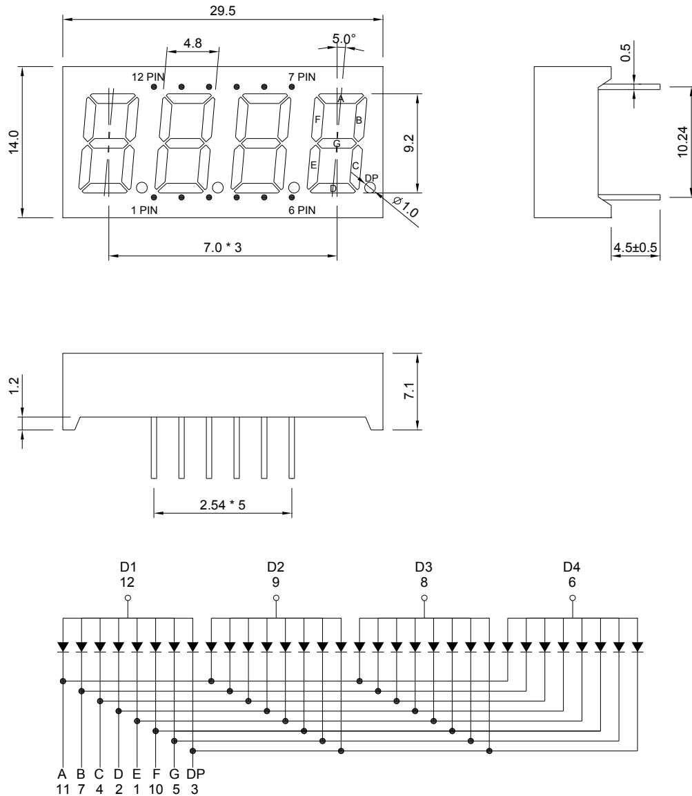
Internal Circuit Diagram
