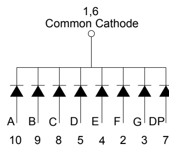
Internal Circuit Diagram
