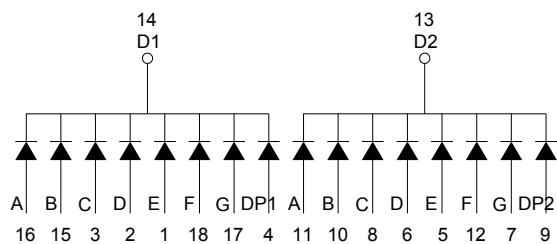
Internal Circuit Diagram
