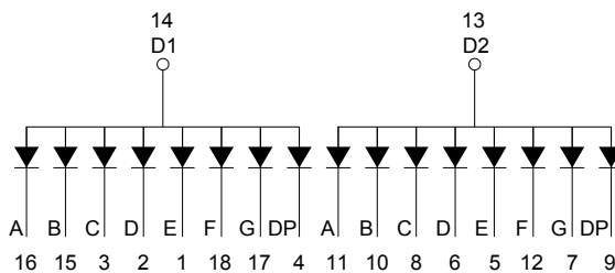
Internal Circuit Diagram
