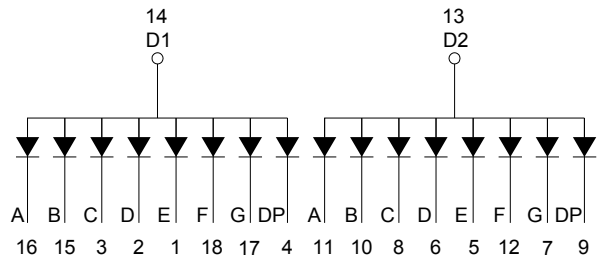
Internal Circuit Diagram
