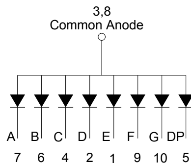
Internal Circuit Diagram
