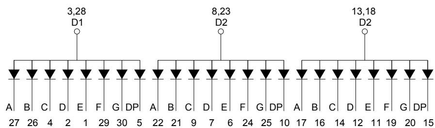
Internal Circuit Diagram
