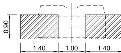
Recommended Soldering Pad
