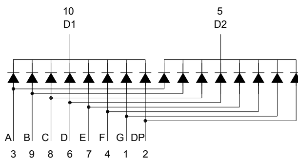
Internal Circuit Diagram
