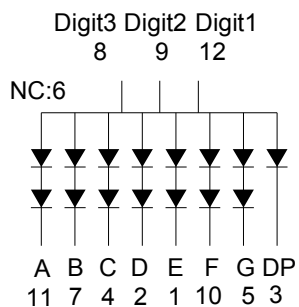
Internal Circuit Diagram
