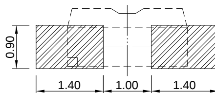
Recommended Soldering Pad
