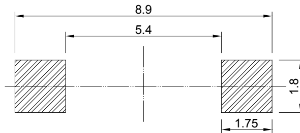
Recommended Soldering Pad
