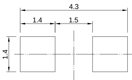
Recommended Soldering Pad
