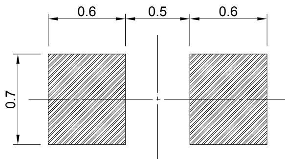
Recommended Soldering Pad
