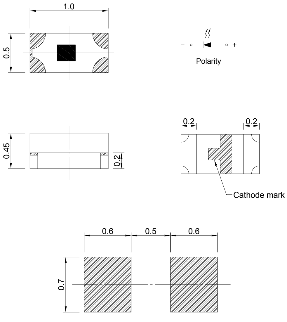
Recommended Soldering Pad
