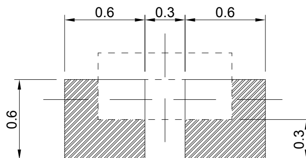
Recommended Soldering Pad
