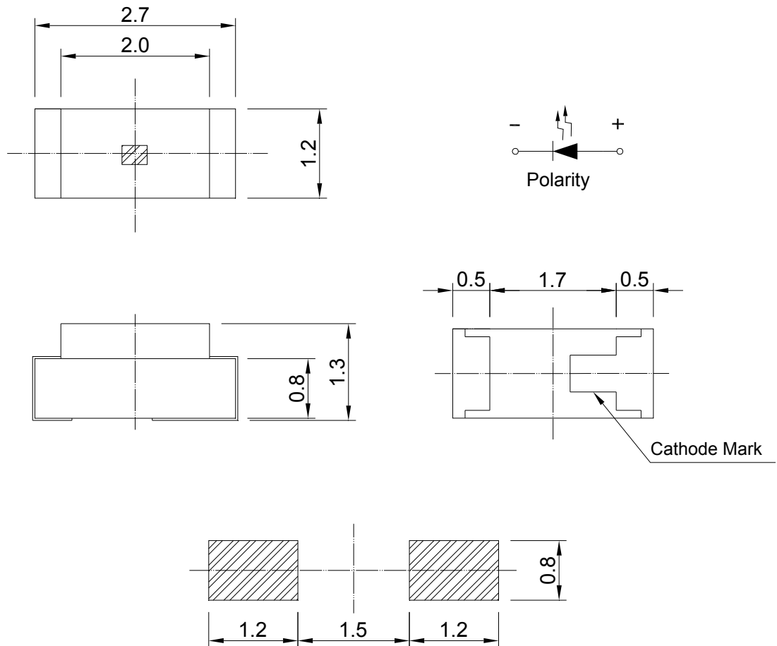
Recommended Soldering Pad
