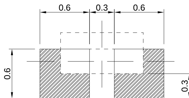
Recommended Soldering Pad
