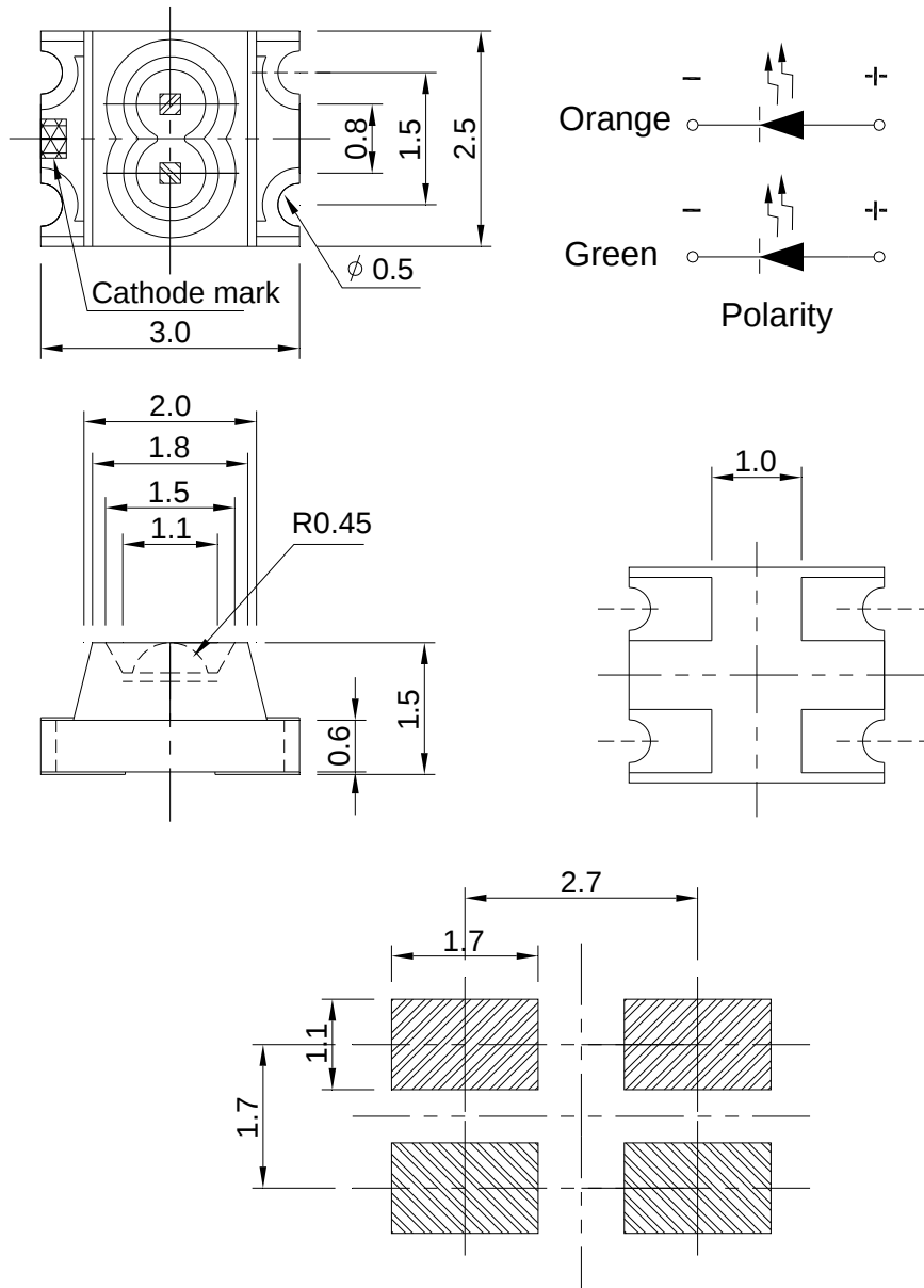
Recommended Soldering Pad
