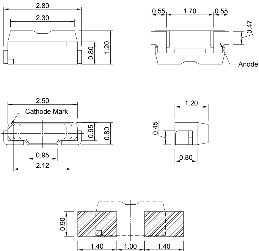
Recommended Soldering Pad
