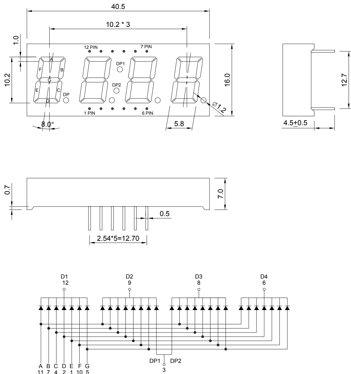
Internal Circuit Diagram
