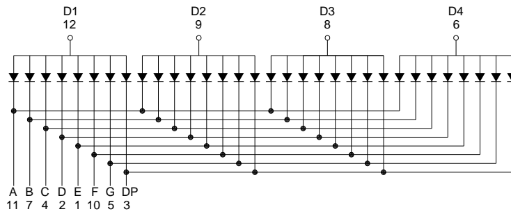
Internal Circuit Diagram
