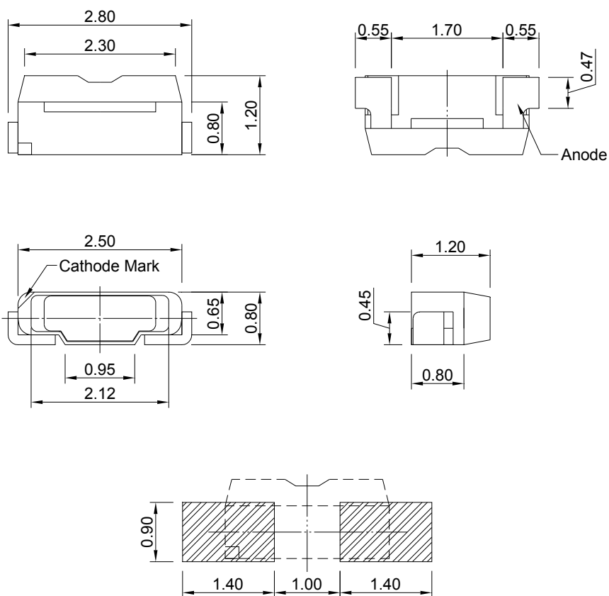
Recommended Soldering Pad
