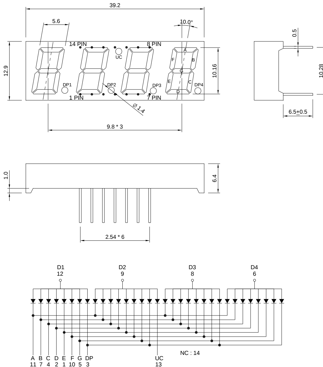
Internal Circuit Diagram
