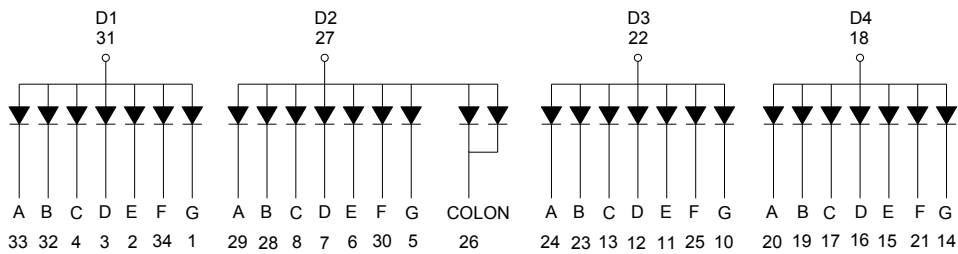
Internal Circuit Diagram
