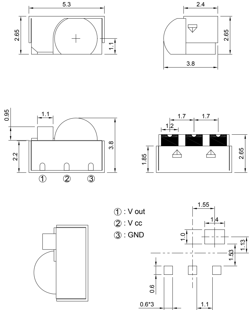
Recommended Soldering Pad
