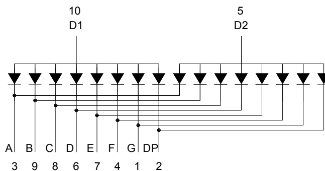
Internal Circuit Diagram
