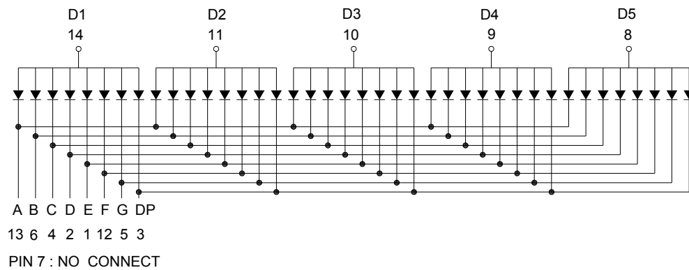
Internal Circuit Diagram
