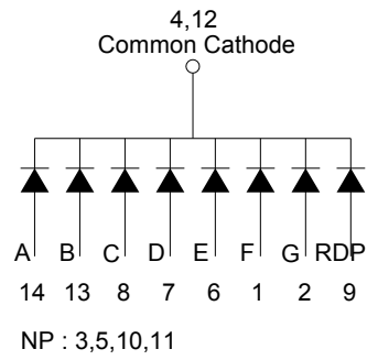
Internal Circuit Diagram
